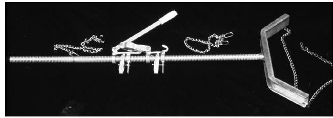
Figure 2. A mechanical calf extractor or puller which permits additional traction in pulling the calf in difficult births. It is designed to span the rear of the pelvis and insures pulling the calf at the correct angle and tension to avoid unnecessary injury to the cow and calf.
